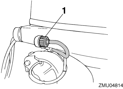
1. Flushing device
