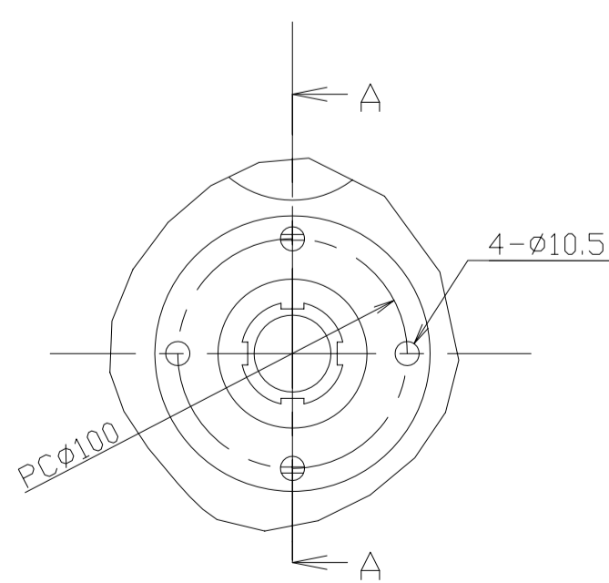
DETAIL OF COUPLING SCALE 1/3
