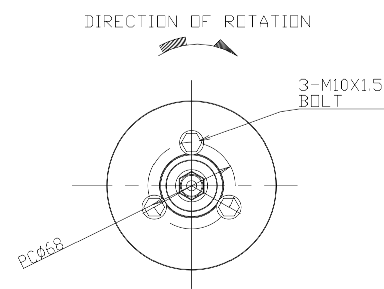
DETAIL OF PULLEY SCALE 1:3 ARROW A
