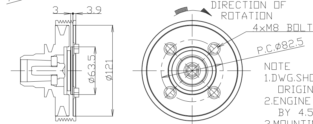
DETAIL OF PULLEY(A) (SCALE 1:3)
