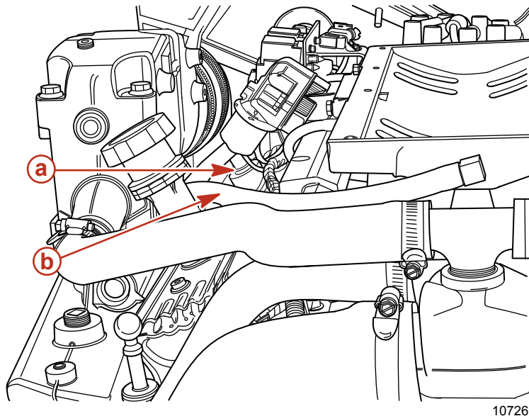
a - PCV valve
