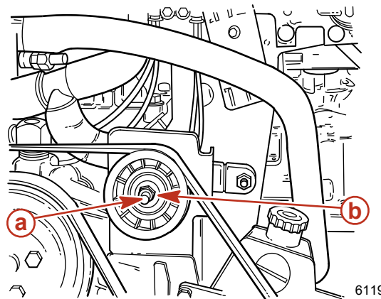
a - 8 mm (1/16 in.) adjusting stud
